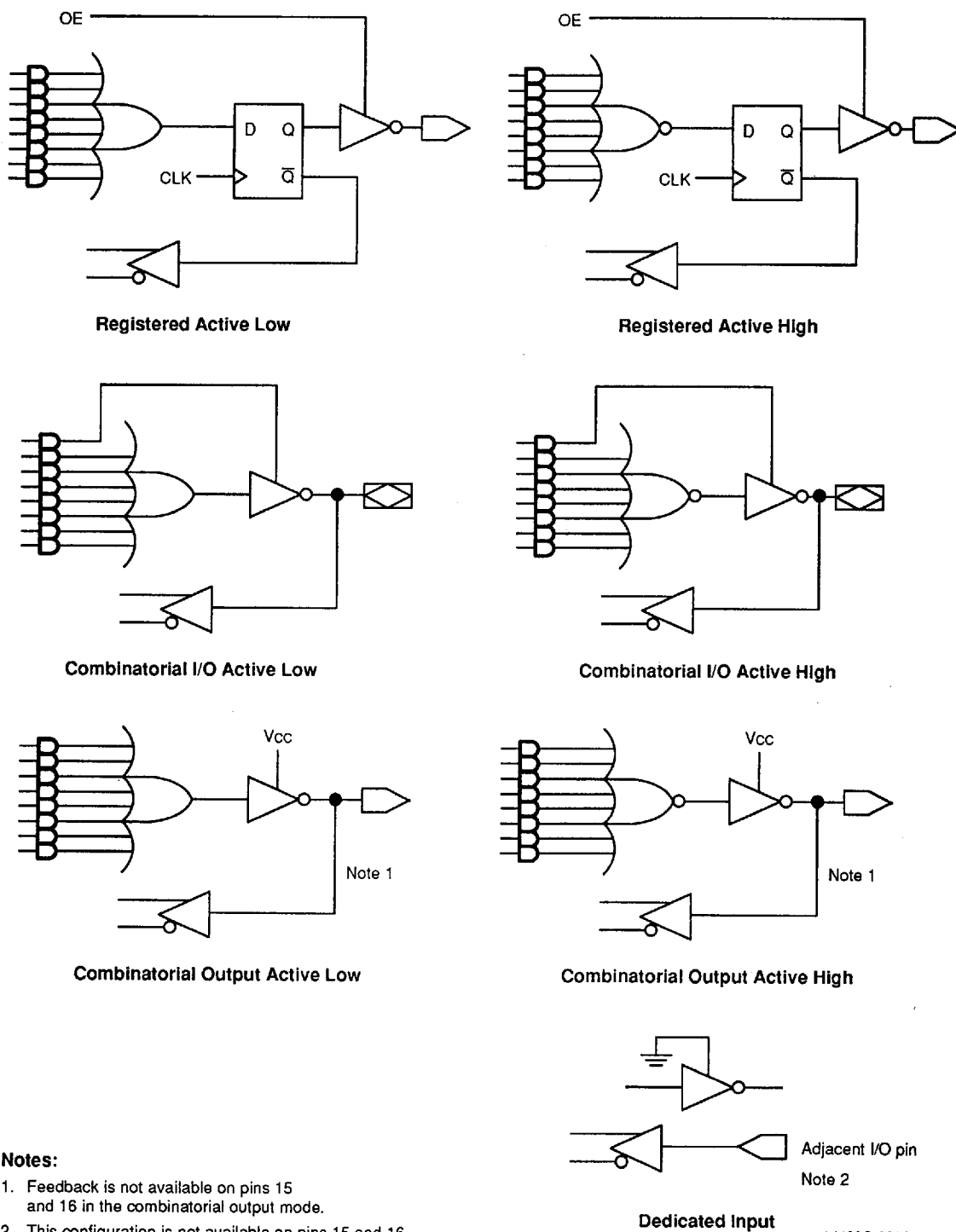
Figure 2. Macrocell Configurations
